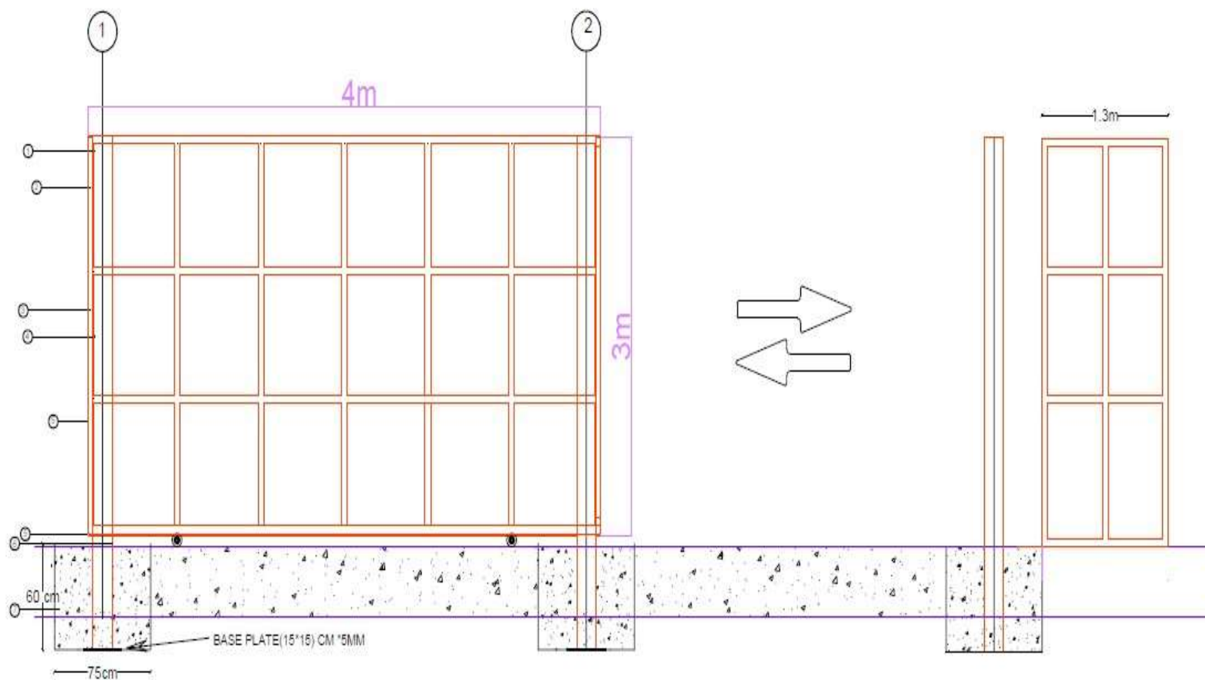
PROFILE PLAN
