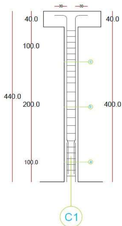
Section(a=c)
