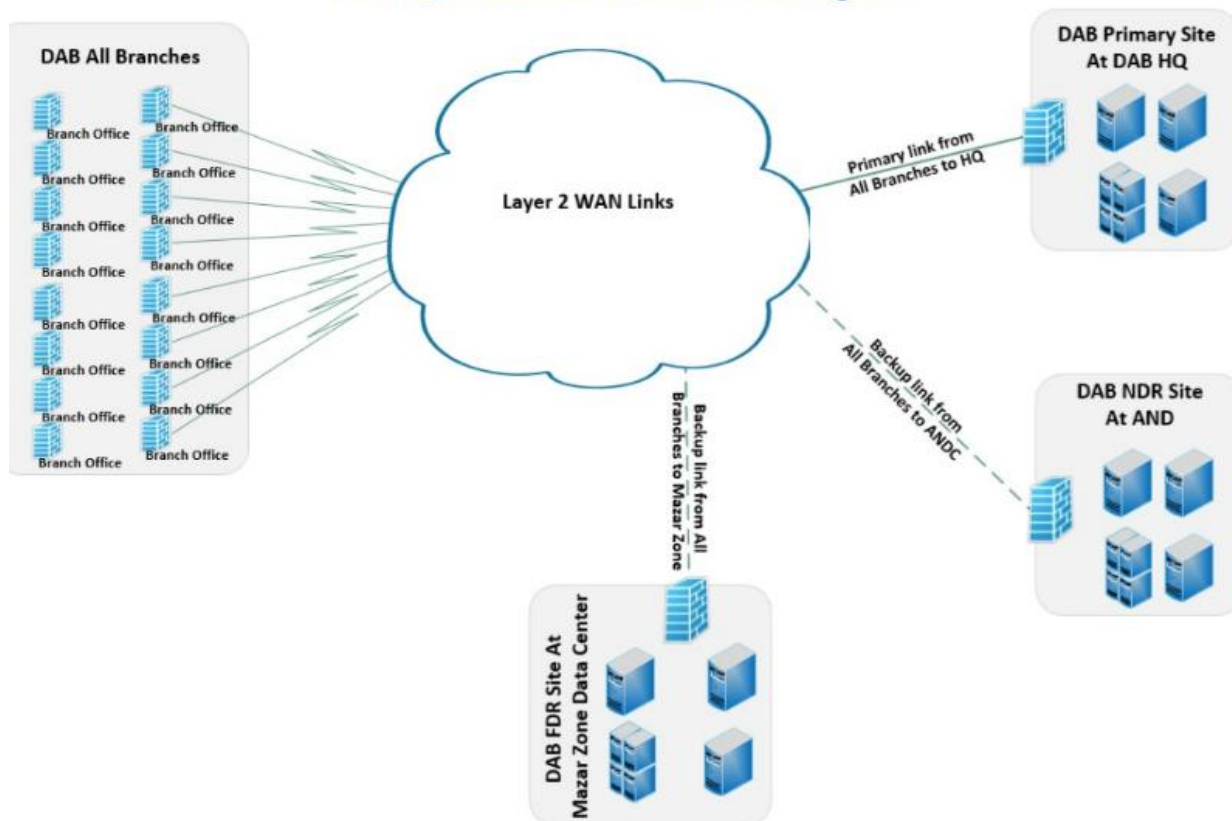
DAB HQ, ANDC and Mazar Zone links Diagram
